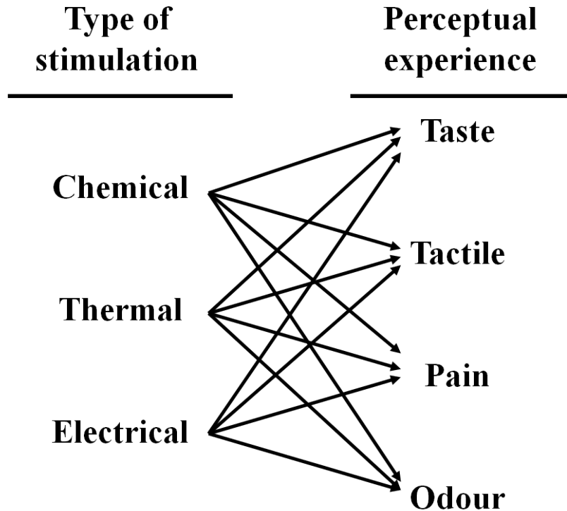
Figure 2: Schematic illustration showing the many-to-many correspondence between sensory inputs and perceptual experiences (see also Iannilli et al., 2008; Nagata et al., 2005).
